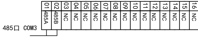
4.3寸一体机MC-20MR-6MT-FE430A-JK3U-A-485接线图
