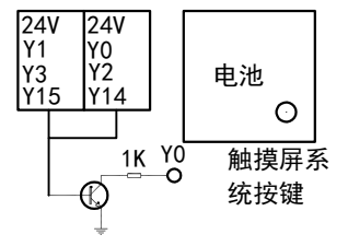
4.3寸一体机MC-20MR-6MT-FE430A-JK3U-E接线图
